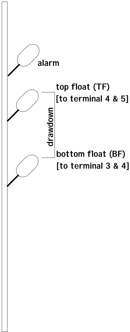
3 Float Configuration (using wide angle floats)
