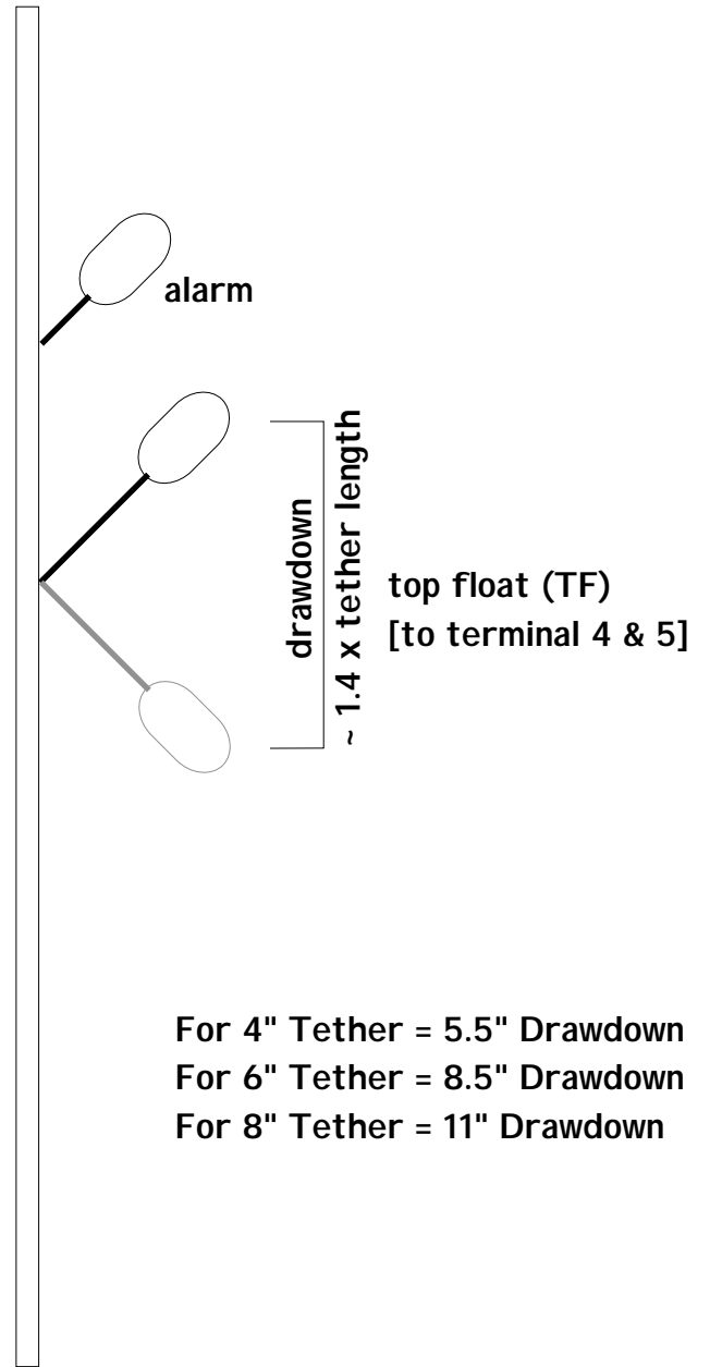
2 Float Configuration (using wide angle floats)
